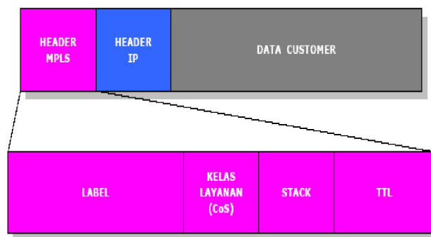
Gambar 1 Header MPLS
